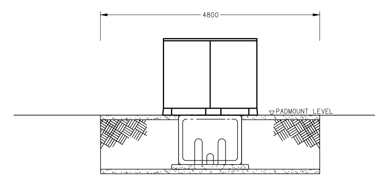
DETAIL B PADMOUNT SECTION VIEW SCALE 1:50
